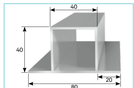
Faltstegprofil • Folding Bar Profile
