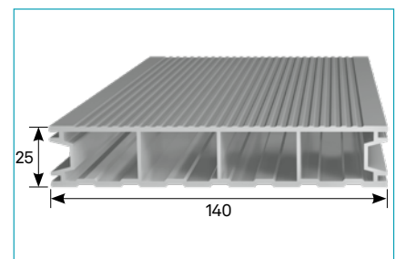
Terrassendiele • Decking Board
