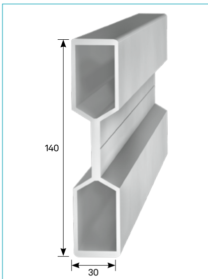
Zarge • Architrave
